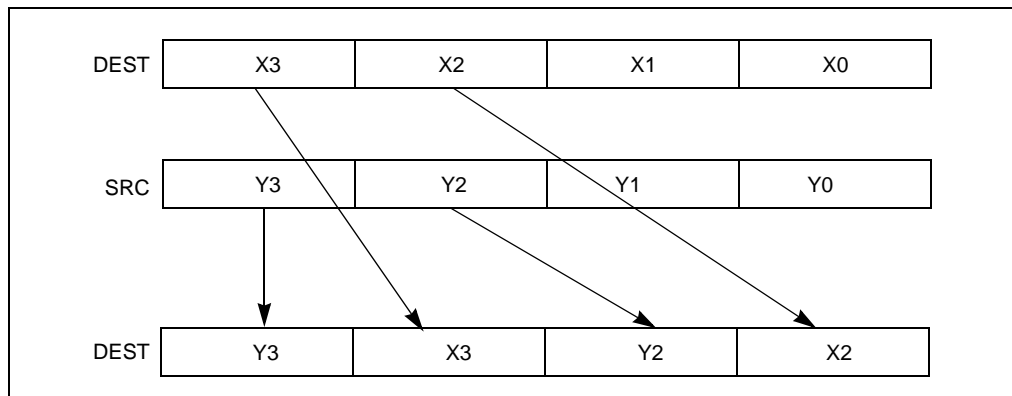
Figure 4-17. UNPCKHPS Instruction High Unpack and Interleave Operation
