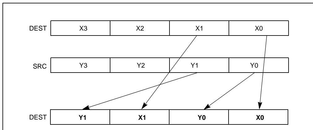
Figure 4-19. UNPCKLPS Instruction Low Unpack and Interleave Operation
