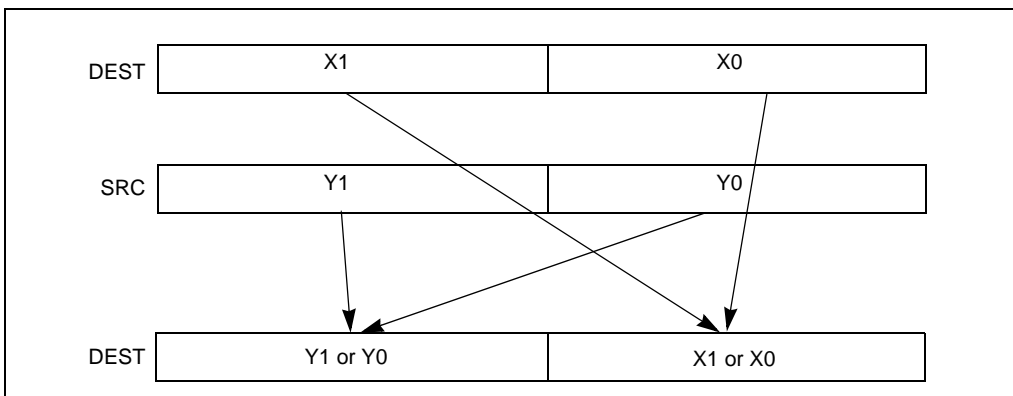
Figure 4-14. SHUFPD Shuffle Operation
