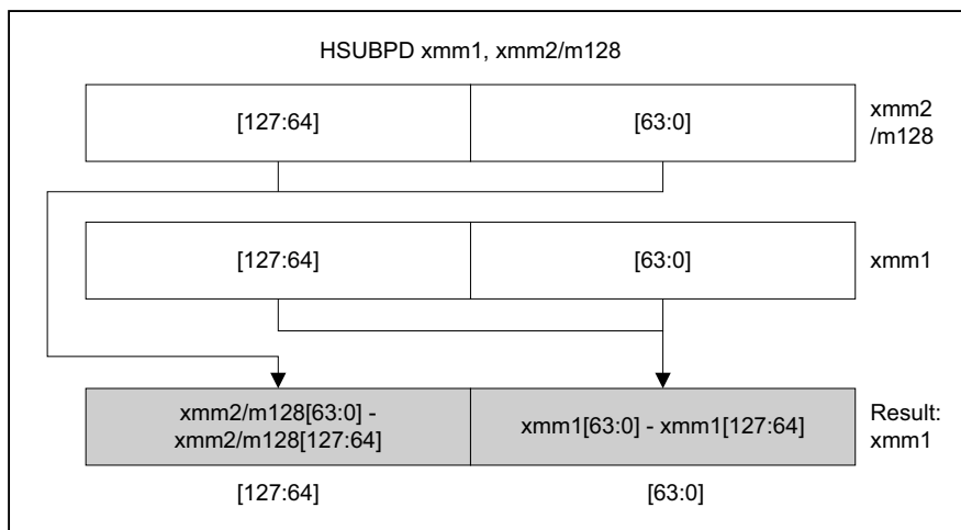
Figure 3-13. HSUBPD—Packed Double-FP Horizontal Subtract
