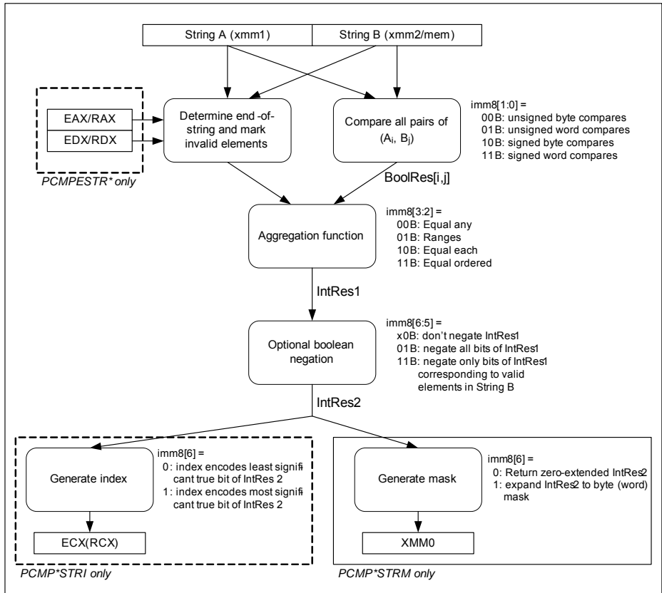
Figure 3-3. Operation of PCMPSTRx and PCMPSTRx
