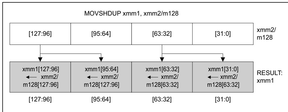
Figure 3-16. MOVSHDUP—Move Packed Single-FP High and Duplicate
